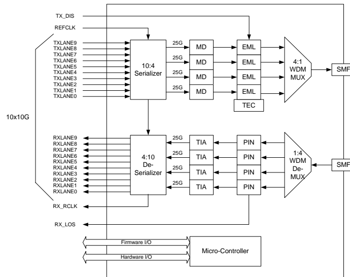
Figure 3- Generation 1 100GBASE-LR4 Implementation Concept
