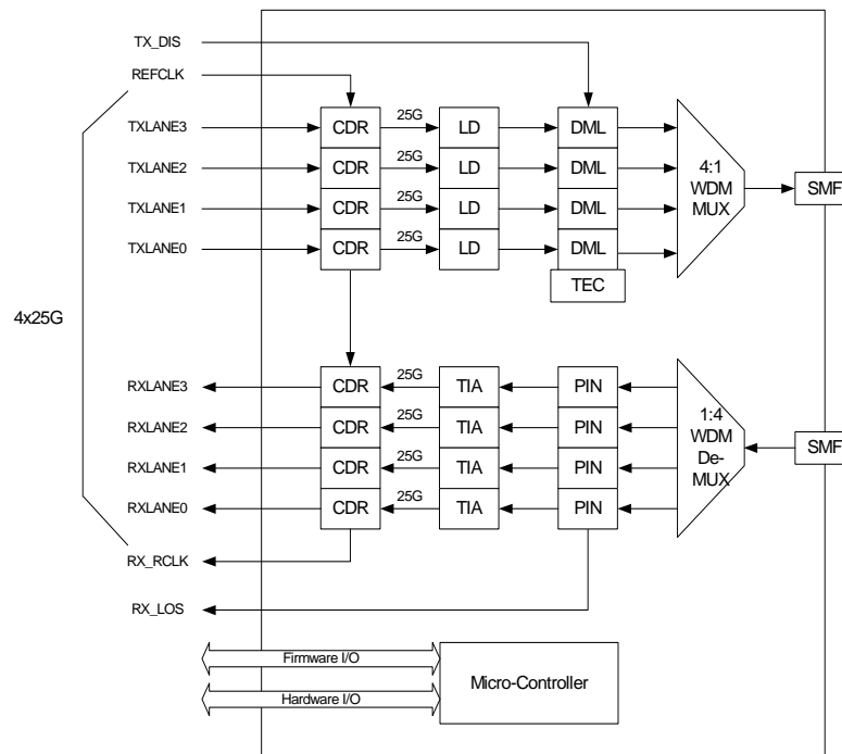
Figure 4- Generation 2 100GBASE-LR4 Implementation Concept
