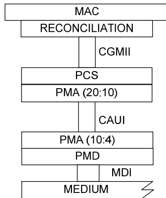
Figure 3 – Potential Implementation for 100GBASE-LR
